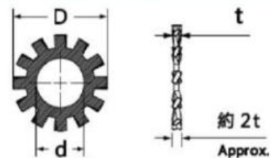
BW型-外齒型墊圈 BW Series External Toothed Lock Washer
