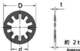
AW型-內齒型墊圈 AW Series Internal Toothed Lock Washer
